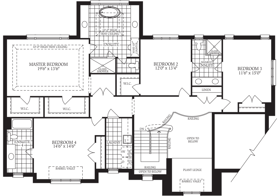
SECOND FLOOR ELEVATION A
